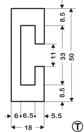
BARANDA C 33
