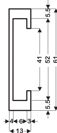
BARANDA C 52
