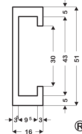
BARANDA C60
